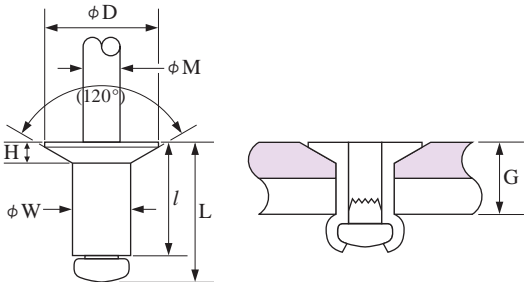
(Countersunk)
