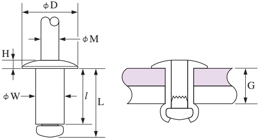
(Round head)
