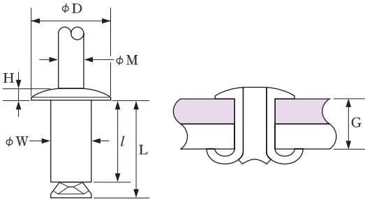
(Round head)
