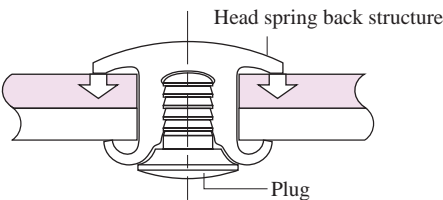
The effect of the plug and the head “spring back structure” prevents loosening of the fastened joint.
