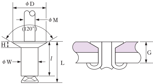
(Countersunk)
